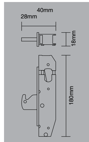
Hook Bolt
