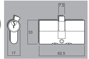
Whitco Pin Cylinder
