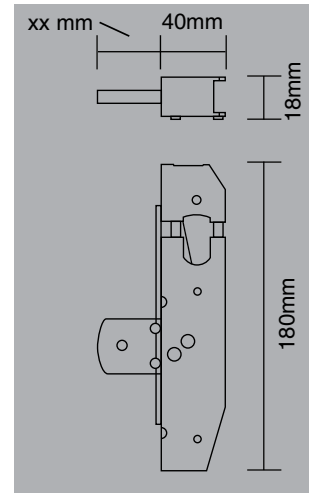
Mortice Lock
