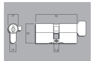
Whitco Cylinder & Turn
