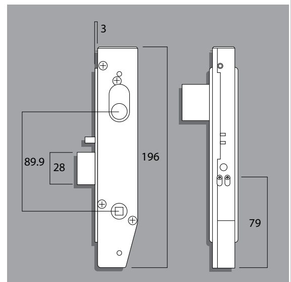
"Y" Cam
